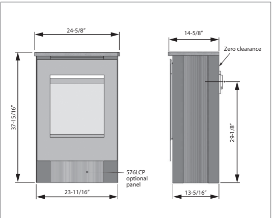
530IL Log Set Engine (shown above) with Lift and Lower Cover Panel (576LCP optional)
