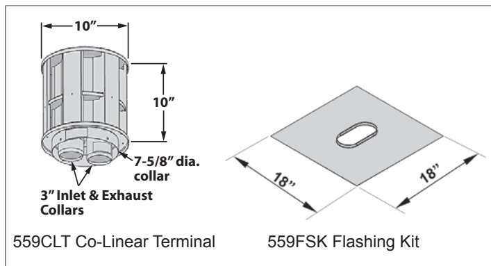
Terminal Cap
